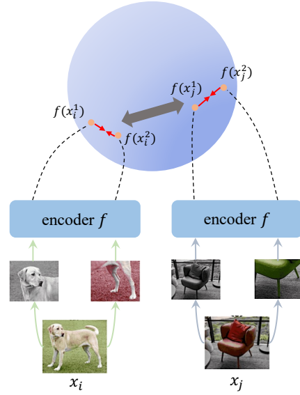
Figure 1. Illustration of contrastive learning on the hypersphere. Red arrows denote positive pairs tend to attract each other, and the gray arrow denotes negative pairs tend to repel each other.
